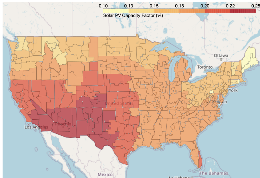
FIGURE 3.1: Capacity factor for solar PV systems in the US.
