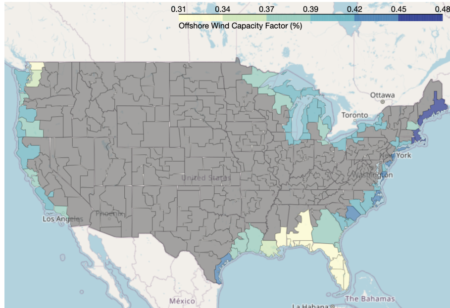
FIGURE 3.3: Capacity factor for offshore wind systems in the US. Grey regions indicate that offshore systems are not feasible.
